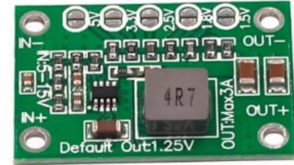
CA-1235 - 12V to 5V Buck Converter
